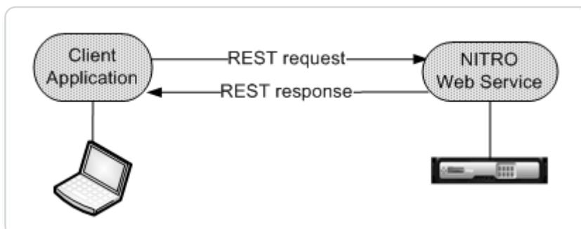
Figure 1. NITRO workflow
